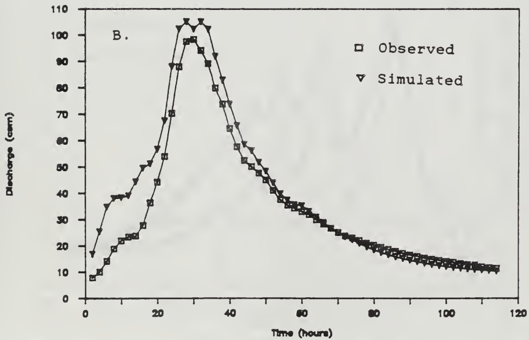
Figure 32. (A) Hyetograph, and (B) simulated and observed hydrographs for a "simple" rainfall event on the Nestucca River, Oregon Coast Range (November 21-29, 1962).
